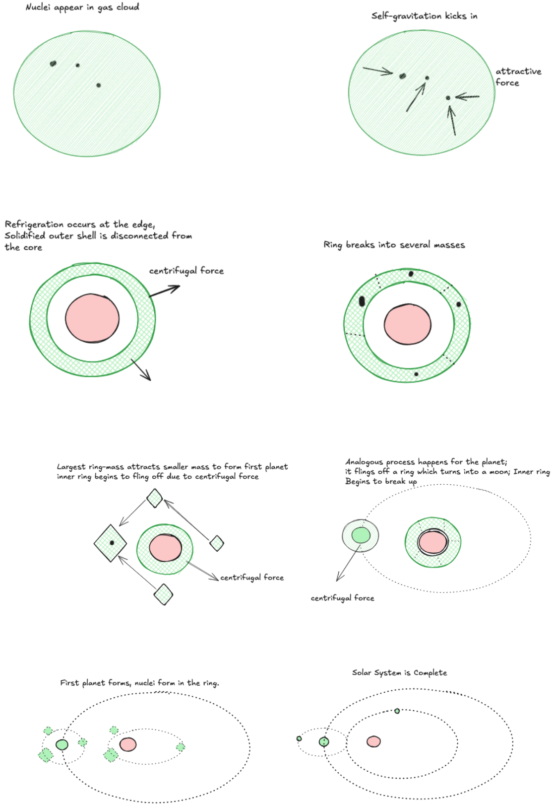
Figure 1: The Nebular Hypothesis: From observed stellar nebulae (top) to planetary condensation (bottom).
