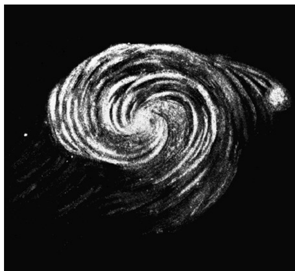
Figure 6: 1845 sketch made by Lord Rosse (William Parsons, 3rd Earl of Rosse) of a Whirlpool Galaxy, based on observations using Leviathan [4].
